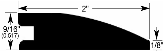
Reducer
