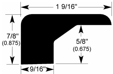
Square Nose Reducer
